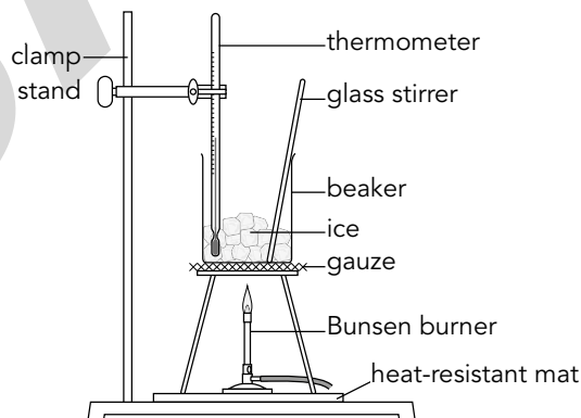
Figure 1.1: Setup for measuring the changing state of ice.
