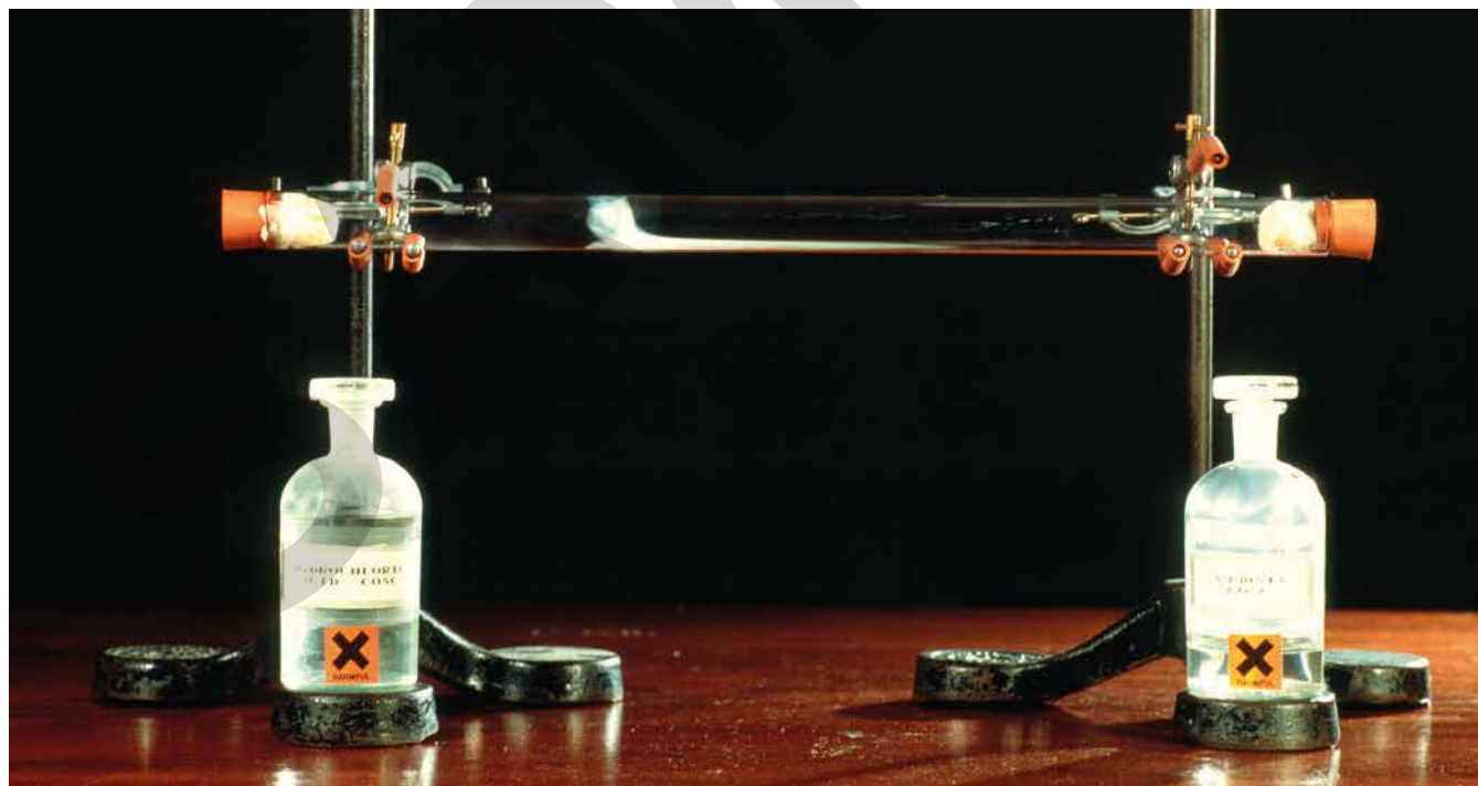
Figure 1.21: Ammonia and hydrochloric acid fumes diffuse at different rates.
