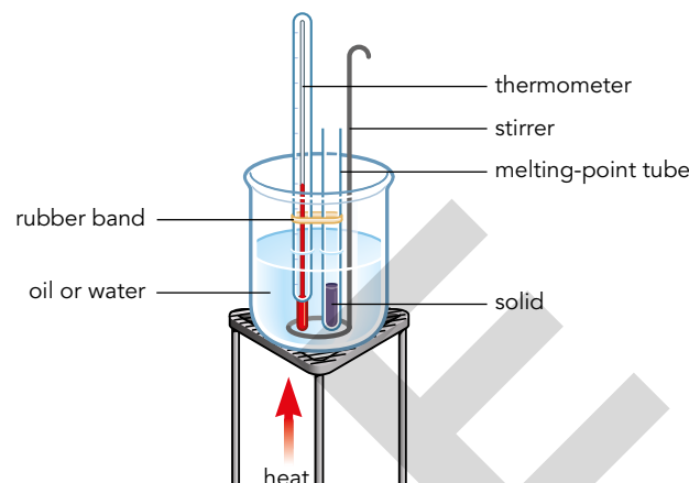
Figure 1.9: Apparatus for measuring the melting point of a solid. A water-bath can be used for melting points below 100^{\circ}\text{C} and an oil bath for melting points above 100^{\circ}\text{C} .
